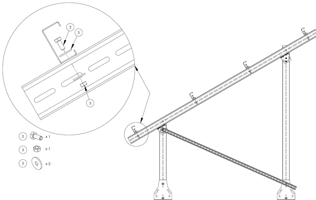
Figure 6. Attachment of Horizontal C-Profiles.
