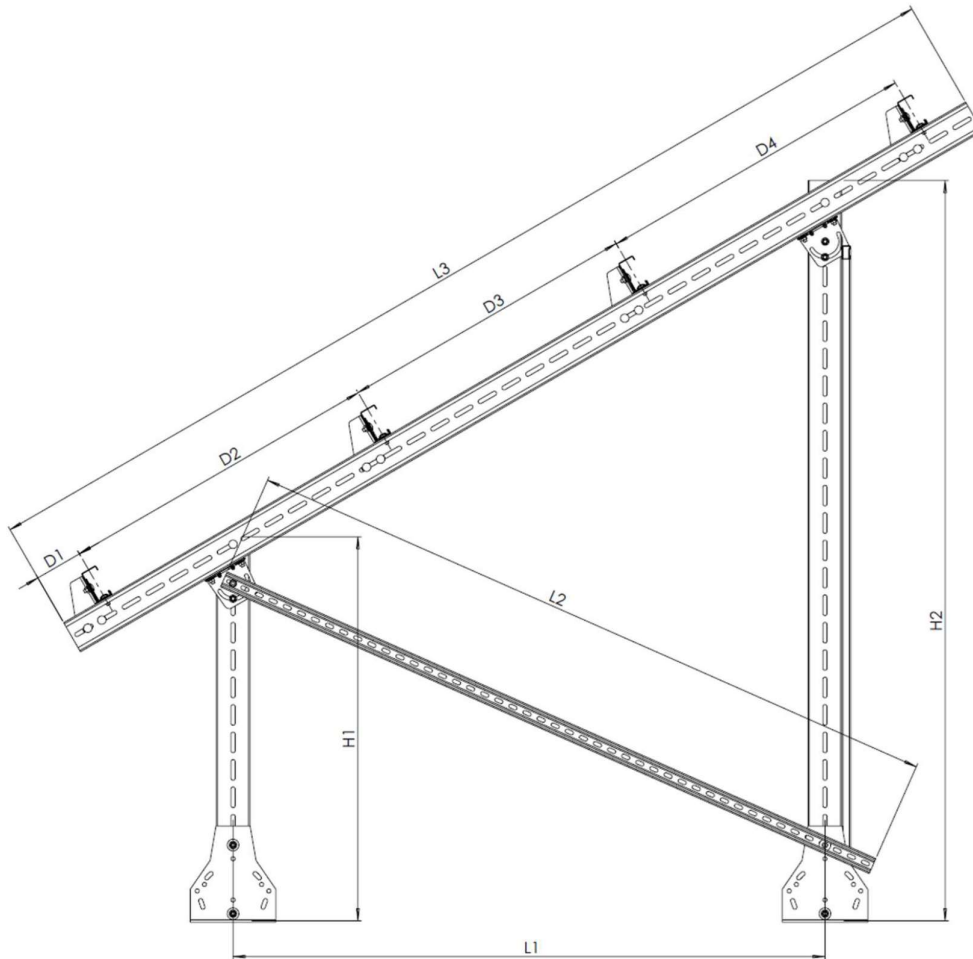
Figure 1. Stand dimensions.
