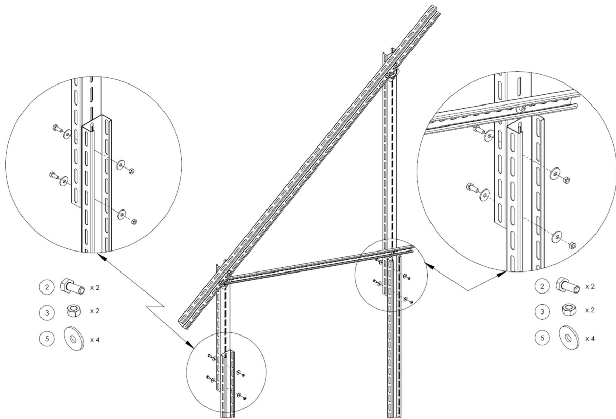
Figure 3. Pile-Mounted leg.
